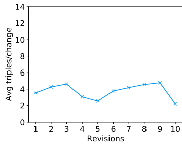
(h) Triple-to-entity changes in Wikidata
