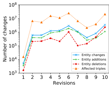
(a) Entity changes for DBpedia
