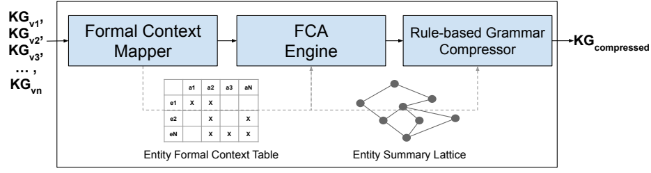
Fig. 2: Zip function: our compression approach creates a formal context from the same entities in different KG deltas. Then, we apply FCA to obtain an entity summary lattice. Finally, we execute a rule-based grammar to produce a compressed KG as output.
