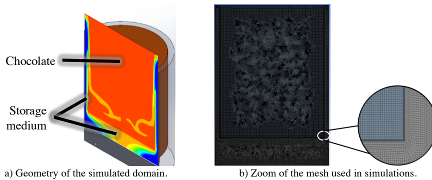
Fig. 5. Geometry built in ANSYS Fluent CFD simulation software. A hexahedral hybrid mesh was used, with 150000 elements and 150000 nodes.
