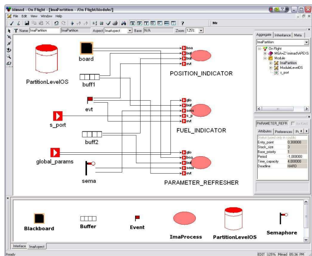
Figure 8: A MIMAD Model of ON_FLIGHT.
