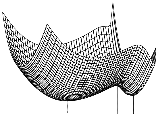
FIGURE 1. Function \phi with one Saddle Point and Two Stable Equilibrium Points. Two classes with \lambda_1 = 0.68 , \lambda_2 = 9.0 , A_1 = 1 and A_2 = C = 20 .
