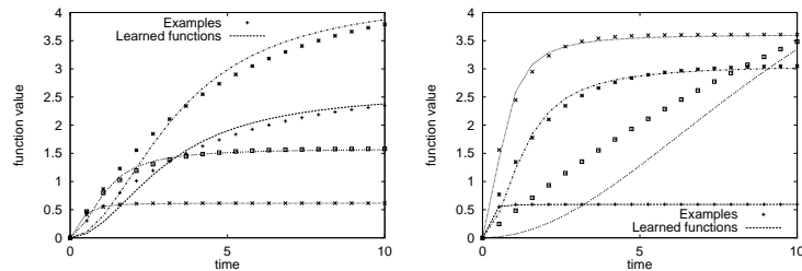
(a) On training examples (b) On test examples Fig. 9. Correct Identification and Generalization with SG-GP
