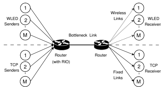
Figure 7: Topology used for testing TCP friendliness.
