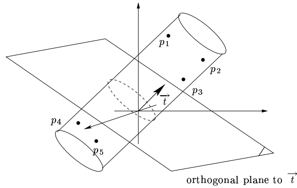
Figure 1: A cylinder through five points
