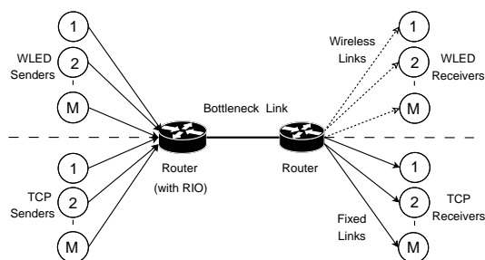
Figure 7: Topology used for testing TCP friendliness.
