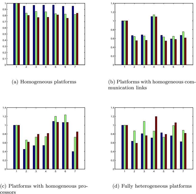
Figure 1: Comparison of the seven algorithms on different platforms.
