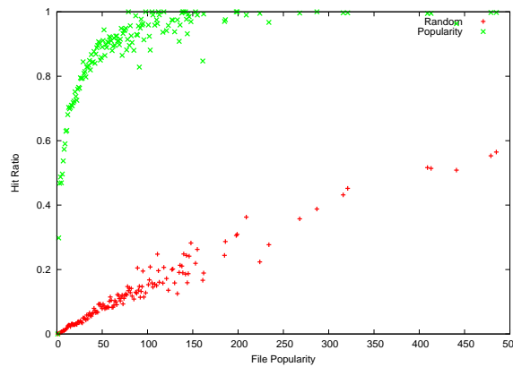
Figure 7: Hit Rate function of File Popularity
