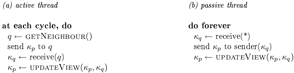
Figure 1: Gossip-based protocol executed by peer p
