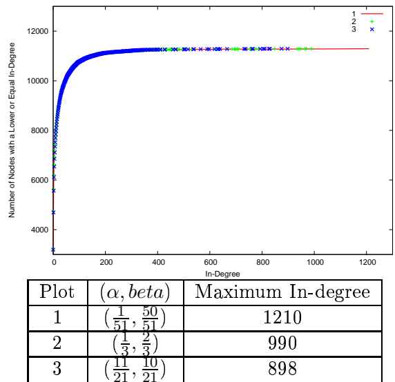
Figure 6: Impact of \alpha and \beta in the Distribution of Peers
