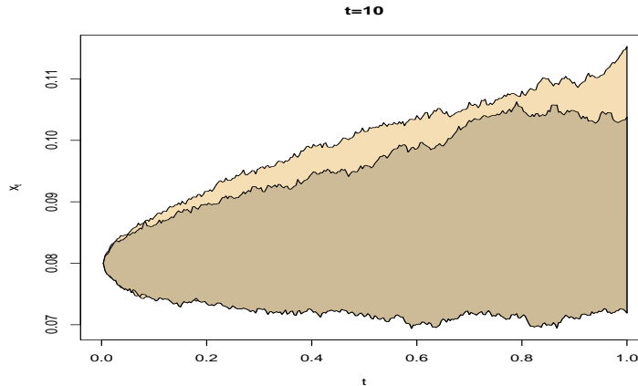
Figure 2: Cox-Ingersoll-Ross European option: range of the simulated process r_{(p+1)T/n}^n ( lighter background ) compared with the resampled process \tilde{r}_{(p+1)T/n}^n ( darker background ) for K = 0.09 , using a D -kernel PMC algorithm with \theta = 0 , \theta = 1 and \theta = 2 , T = 10 iterations and N = 10,000 simulations.
