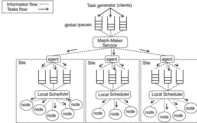
Figure 2: The DIRAC scheduling model.
