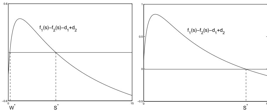
Figure 2: Geometric interpretation of (F3) : Graph of the function f_1 - f_2 - d_1 + d_2 , with d_1 > d_2 (Left) and d_1 \leq d_2 (Right)
