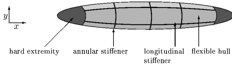
Figure 1: Prolate structure and stiffeners position
