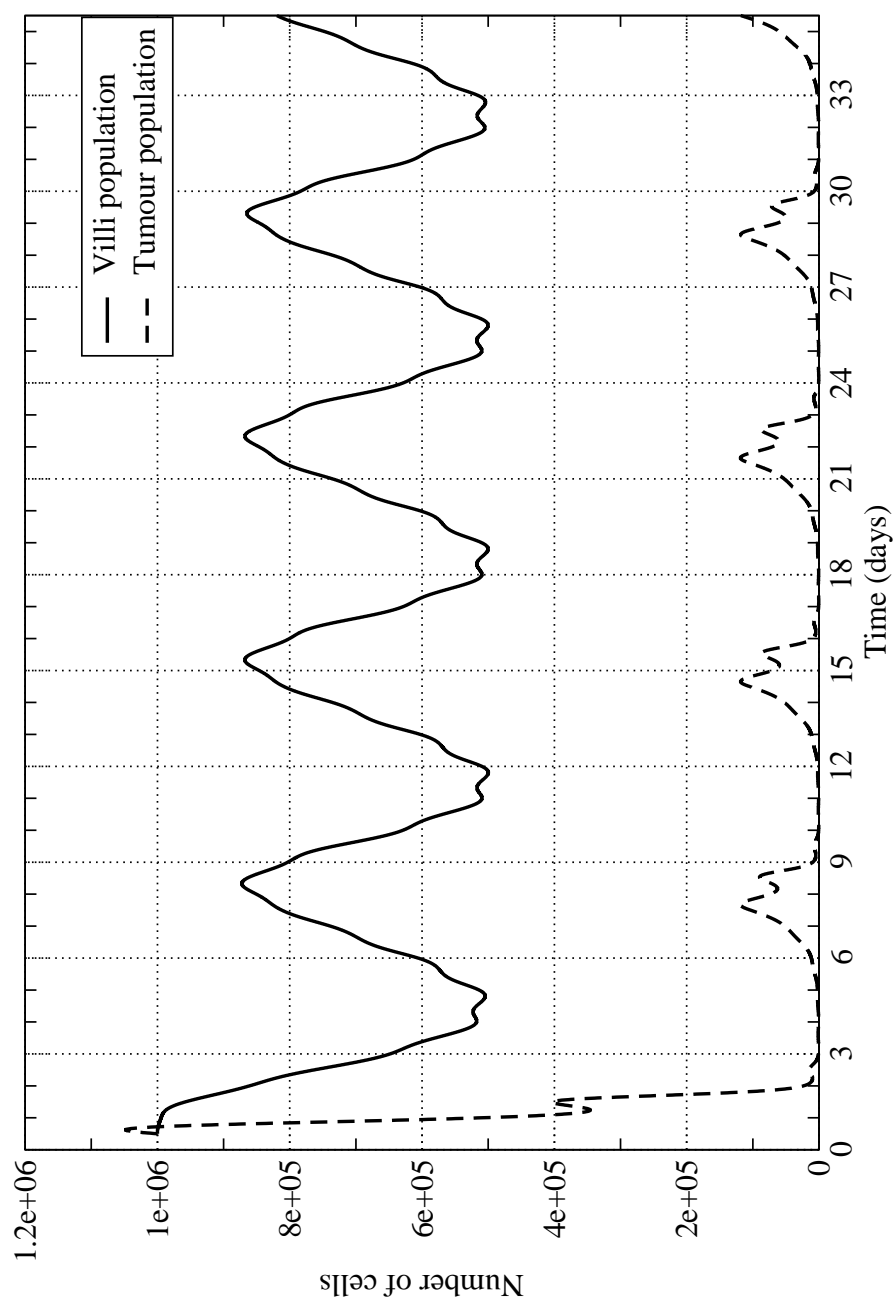
Figure 6: Five weeks containment treatment with 2+5 days cycle: cell populations for \tau_A = 0.5 .
