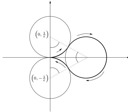
Figure 1: The teardrop trajectory of size 1/\varepsilon .
