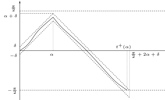
Figure 3: The graph of \theta^+(\cdot, \alpha) .
