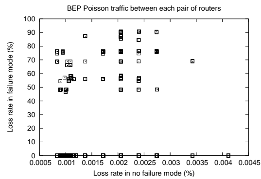
Figure 19: Losses for BEP traffic: failure mode versus no failure mode.
