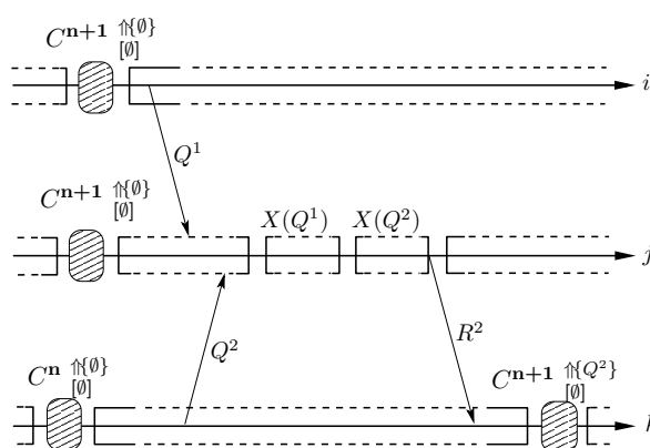
Figure 6: An alteration of the reception order of Q^1 and Q^2 may modify R^2 .
