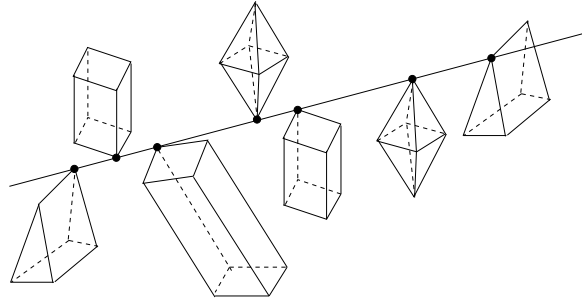
Figure 2: A line tangent at a vertex of each of k polytopes.
