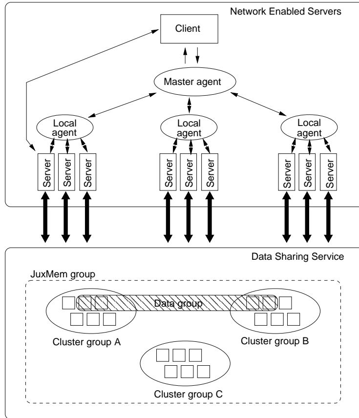
Figure 6: Overall architecture of the grid data-sharing service.
