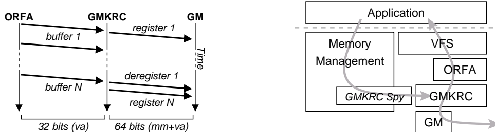
(a) GMKRC principles. Deregistration is delayed. The virtual address ( va ) is prefixed with the address space pointer ( mm ).
