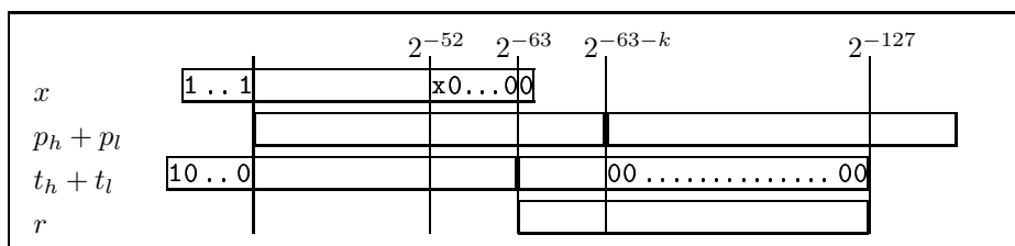
Figure 3: Case when the exponent of t_h is 1 plus that of x . Here the magnitudes are relative to the exponent of t_h .
