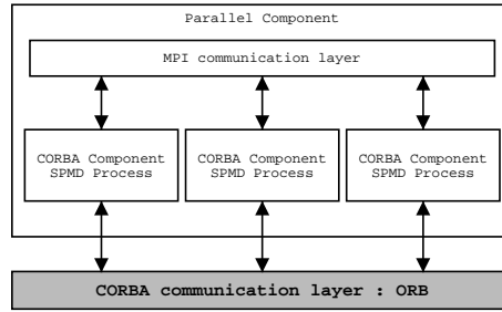
Figure 3: Parallel component concept.
