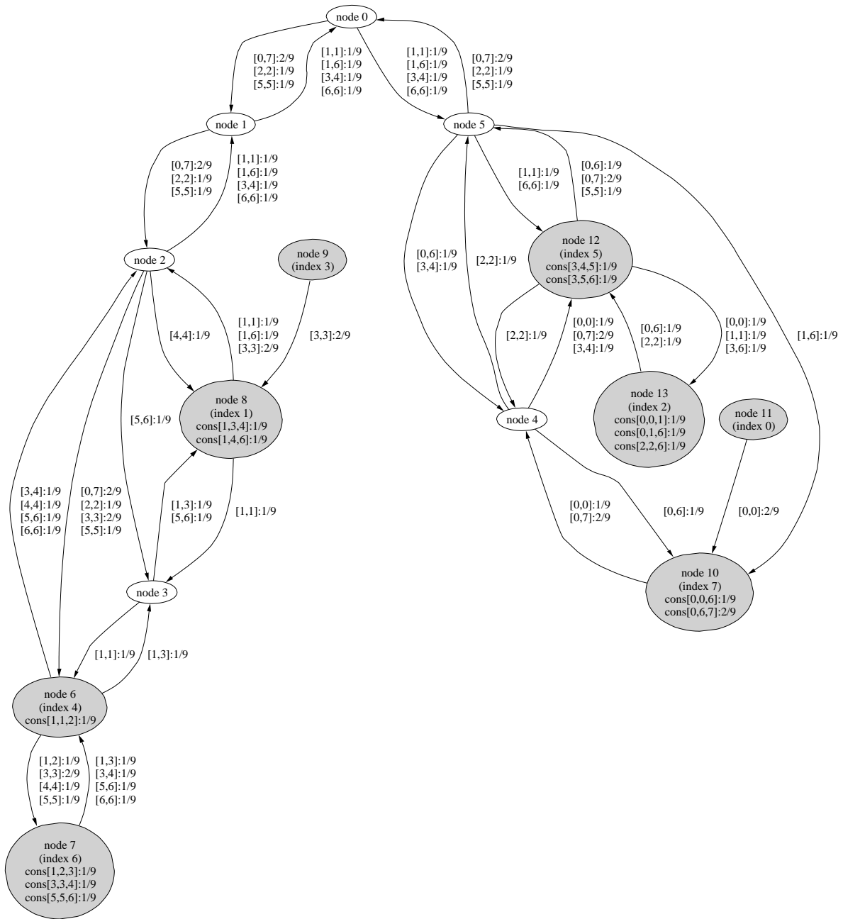
Figure 10: Results of the linear program. The target node is node 6 with index 4. Each link is labeled with the transfers scheduled through it during one time-unit. For example, [1, 6] : 1/9 means that 1/9 message of type v_{[1,6]} pass through the edge during one time-unit. In the same way, the computing nodes are labeled with the tasks which they execute.
