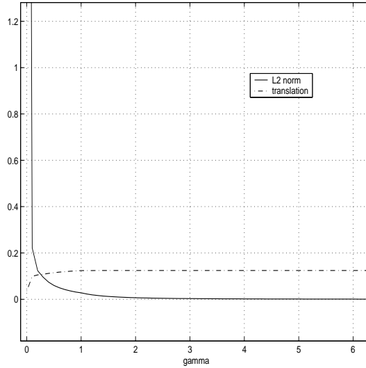
Figure 7: \gamma dependance
