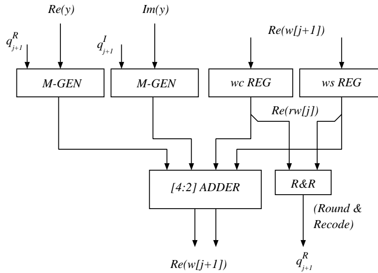
Figure 1: Implementation of recurrence for real part (Similarly for imaginary part). This corresponds to radix-2 or radix-4 schemes. For higher radices, multiple generators (M-GEN) are replaced by digit-vector multipliers producing redundant products, and the [4:2] adder is replaced by a [6:2] adder.
