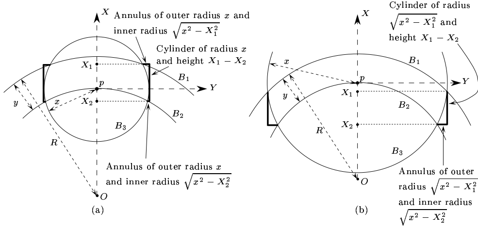
Figure 18. For the proof of Proposition 37, case 1.
