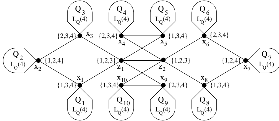
Figure 6: The graph G_5 and its list assignment L_5 .
