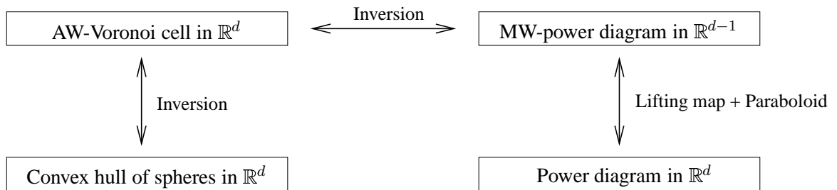
Figure 1: Equivalence relationships between the various Voronoi diagrams.
