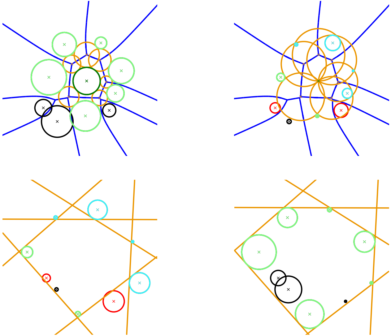
Figure 2: The equivalence relationship between additively weighted Voronoi cells and convex hulls of spheres in two dimensions. P_0 is shown in dark green. Light green and black spheres have positive weight. Light blue and red spheres have negative weight. Light green and light blue spheres correspond to neighbors of P_0 in V_+(\mathcal{E}) . Black and red spheres do not correspond to neighbors of P_0 in V_+(\mathcal{E}) . Top left: the set \{P_0, \dots, P_n\} . The Voronoi spheres U_k of V -dimension 0 are shown in yellow. The Voronoi skeleton is shown in blue. Top right: the set \{P'_0, \dots, P'_n\} . The spheres U'_k are in yellow. The Voronoi skeleton remains the same and P'_0 is a point. Bottom left: the set \{\Sigma_1, \dots, \Sigma_n\} . The hyperplanes \Pi_k are in yellow. Bottom right: the set \{\Sigma'_1, \dots, \Sigma'_n\} . The hyperplanes \Pi'_k are in yellow.
