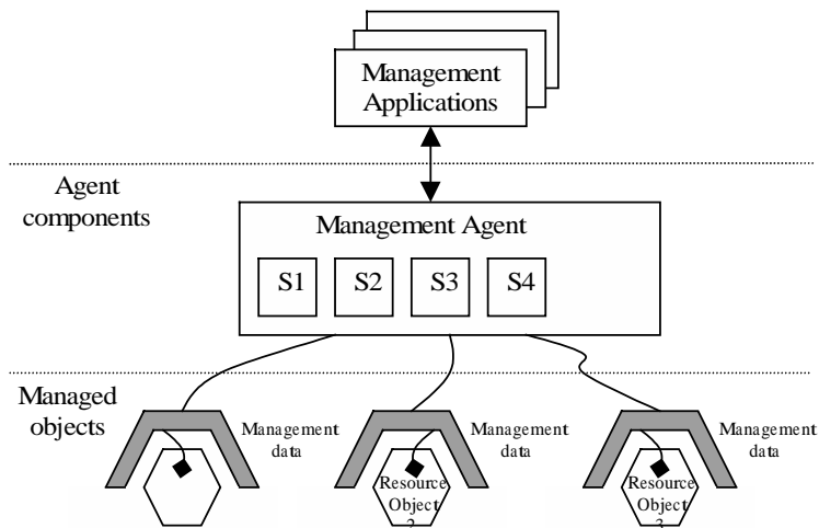
FIG. 1 – Manage/Agent architecture model
