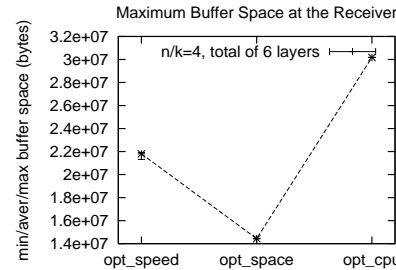
(b) Maximum buffer space
