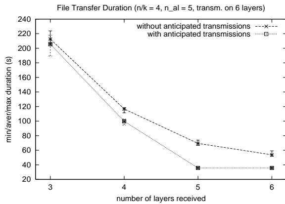
(a) Transfer duration
