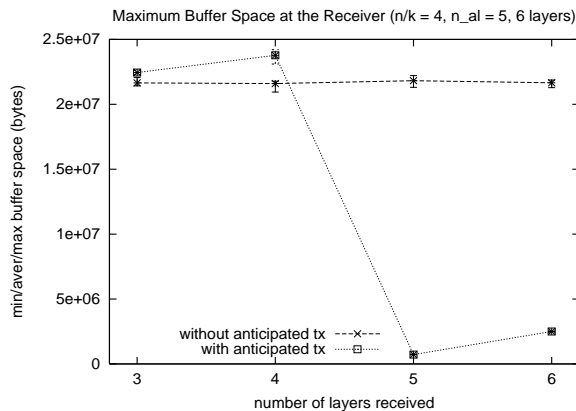
(b) Maximum buffer space
