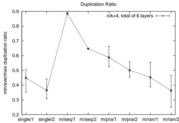
Figure 11: Duplication ratio with various transmission schemes (no loss, \sim 1 MB file).
