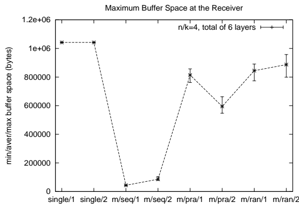
Figure 12: Maximum buffer space at the receiver with various transmission schemes (no loss, \sim 1 MB file).
