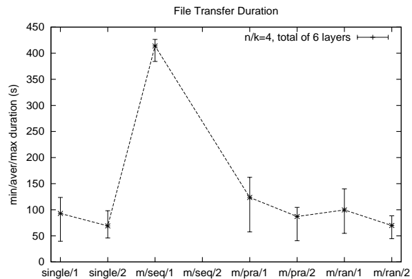
Figure 13: Transfer duration with various transmission schemes (bursty random 1%/75% losses, \sim 1 MB file).
