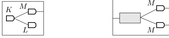
Figure 11: The action graph K \cdot c \cdot (M \otimes L) and the context {}_{-1,1} \cdot c \cdot (M \otimes M)
