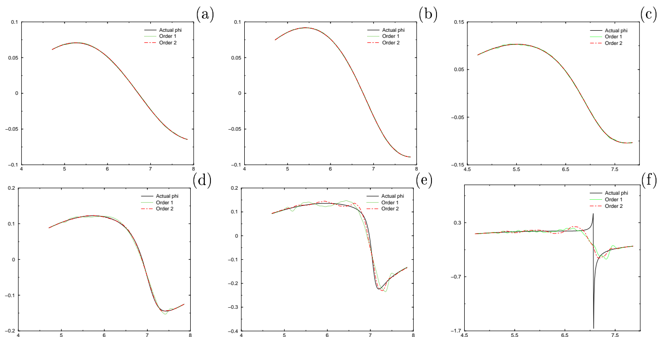
Figure 2: Recovered \varphi for different values of \delta = d(a, \mathbb{T}) : \delta = 4 (a), \delta = 2 (b), \delta = 1.5 (c), \delta = 1 (d), \delta = 0.8 (e), \delta = 0.708 (f) at orders 1 and 2
