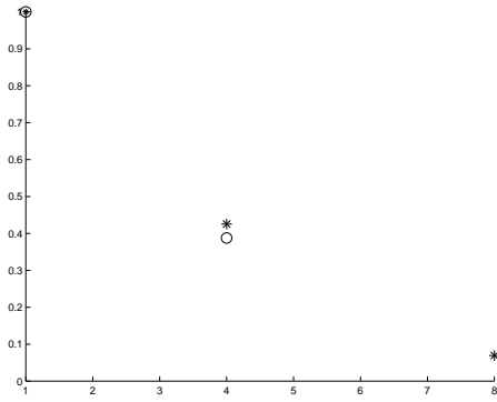
Figure 24: Cuts corresponding to the largest absolute values of the computed refinement indicators
