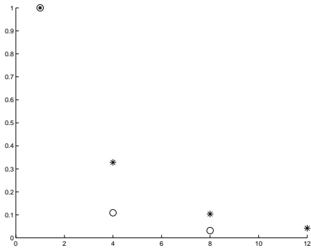
Figure 25: Estimated partition and transmissivity obtained when using a variant of the algorithm
