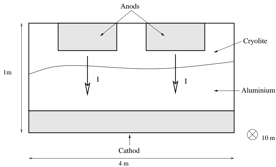
Figure 1: Schematic representation of an aluminium cell
