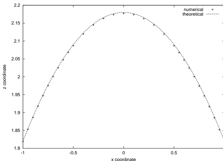
Figure 9: Elevation of the steady state top surface in the simulation of Section 7.2. Comparison between theoretical and numerical results.
