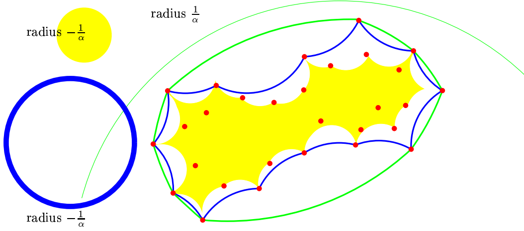
Figure 1: Two \alpha -hulls of a set of points
