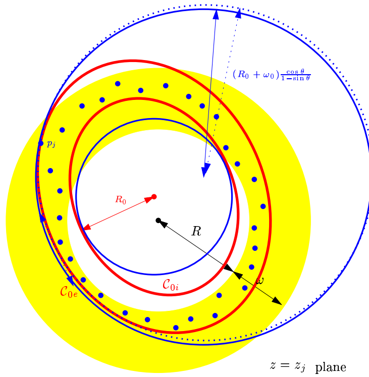
Figure 5: For the proof of Lemma 7
