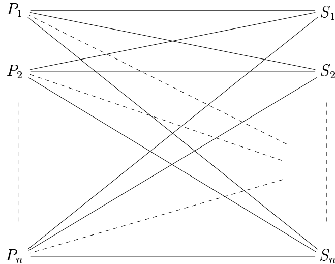
Figure 5: Bipartite graph for MaxTasks1(T).
