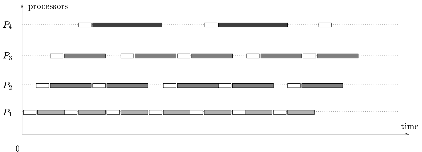
Figure 12: Execution with the greedy algorithm.
