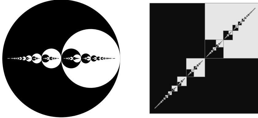
FIGURE 2. Basic continued fractions: the fundamental intervals represented by their supporting discs (left) and the fundamental squares (right). The events [L = k] for ranks k = 0..5 are alternately represented by dark and light colours.
