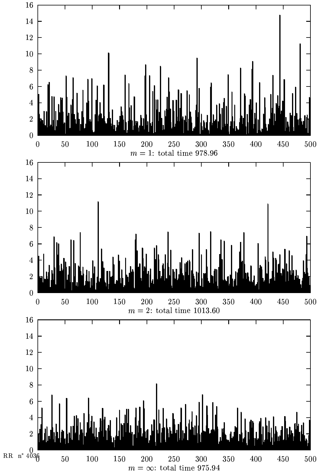
Figure 1: Simulations of 500 successive interarrival times for \rho = 0.5 , \mu = 1 , various m .
