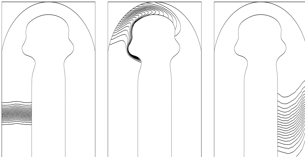
Figure 9: Second class of optimized shapes for the 180 degree turn. Here again, larger curvature variation introduces more dispersion in the advection band away from walls.
