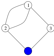
Fig. 1. Multigraph with 4 vertices
