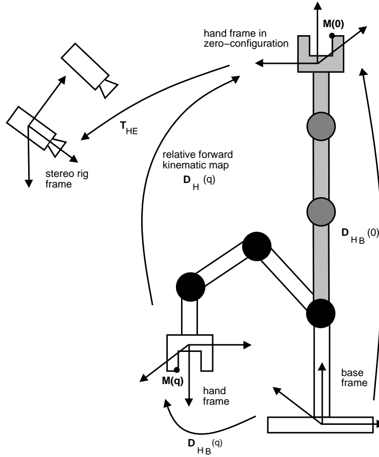
Figure 4: The stereo rig observes the robot in various configurations: a zero-configuration and a general configuration characterized by the vector q of joint variables. The Cartesian frame illustrated on this figure ARE NOT used. Instead, the projective approach uses points physically attached to the end-effector and observed by both cameras.
