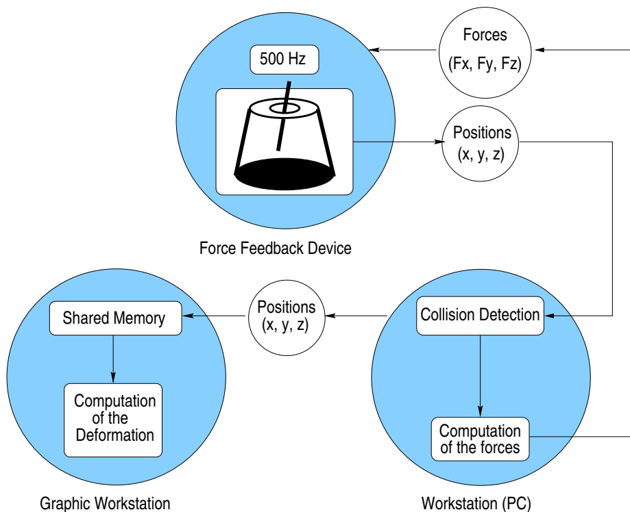
Figure 6: Example of simulation systems.
