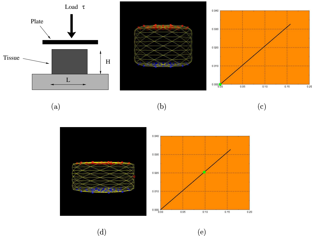
Figure 3: Behavior of linear elastic materials.
