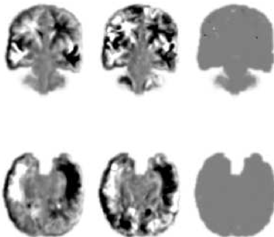
Figure 10: Dissymmetries between a population of 10 right handed males and a population of 3 left handed males. Left: average of the 10 \|F\|div(F)\| right handed maps; middle: average of 3 left handed; right: significance map for \alpha_0 = 0.001 ; the same significance level as for figure 9. These preliminary results are not conclusive with respect to a significant morphological difference between left and right handed people. Larger datasets are probably requested before drawing any conclusion.
