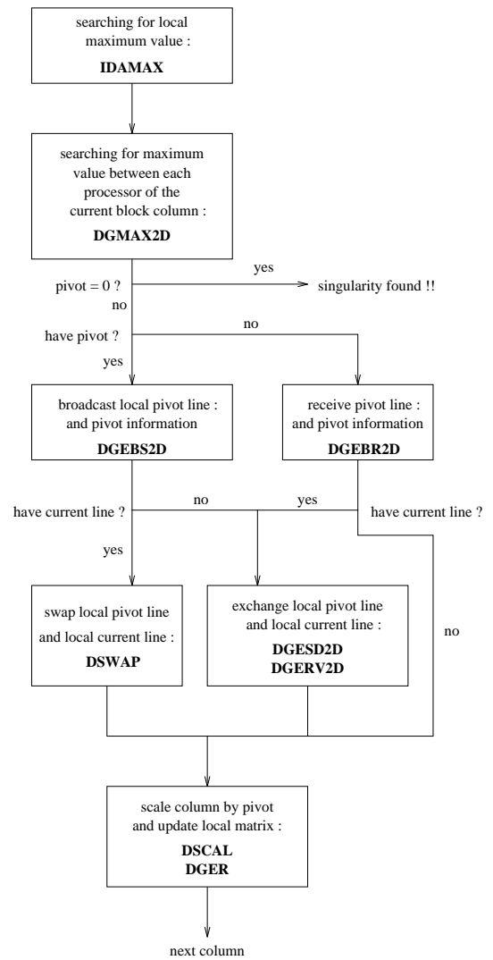
Figure 5: Execution scheme of the PDGETF2 routine.
