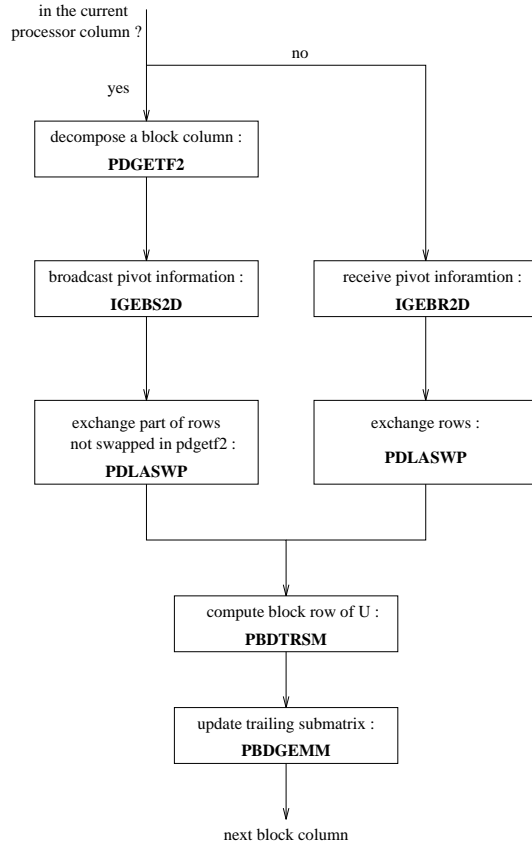
Figure 4: Execution scheme of the PDGETRF routine.
