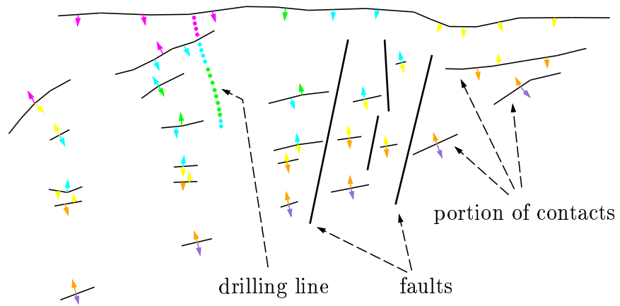
Figure 27: Initial data.
