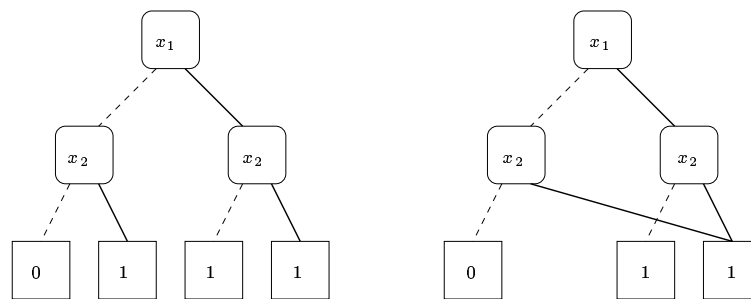
Figure 1: Two BDD representations of f(x_1, x_2) = x_1 + x_2 . Each node represents a test over one variable. Solid lines represent the “then” branches, dotted lines the “else” branches. The representation on the left is the complete tree corresponding to the Boole-Shannon expansion of f , whereas the diagram on the right is more compact.
