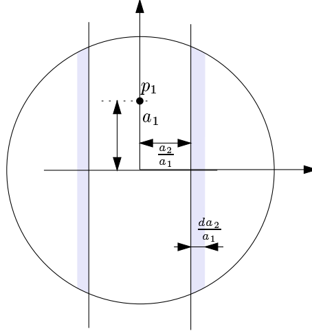
Figure 1: For the analysis of the 2-determinant
